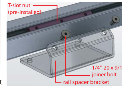
Rail Spacer Bracket / Mid Base Attachment Detail
