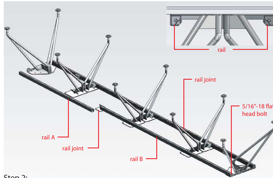
Rail Joint Detail
