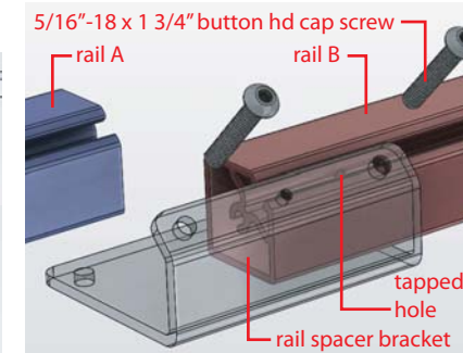
Rail Joint Detail
