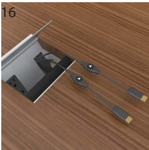
16 Pass "Show Me" cables through Forum face and plug into Switcher Box.
