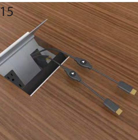
15 Pass "Show Me" cables through Forum face and plug into Switcher Box.
