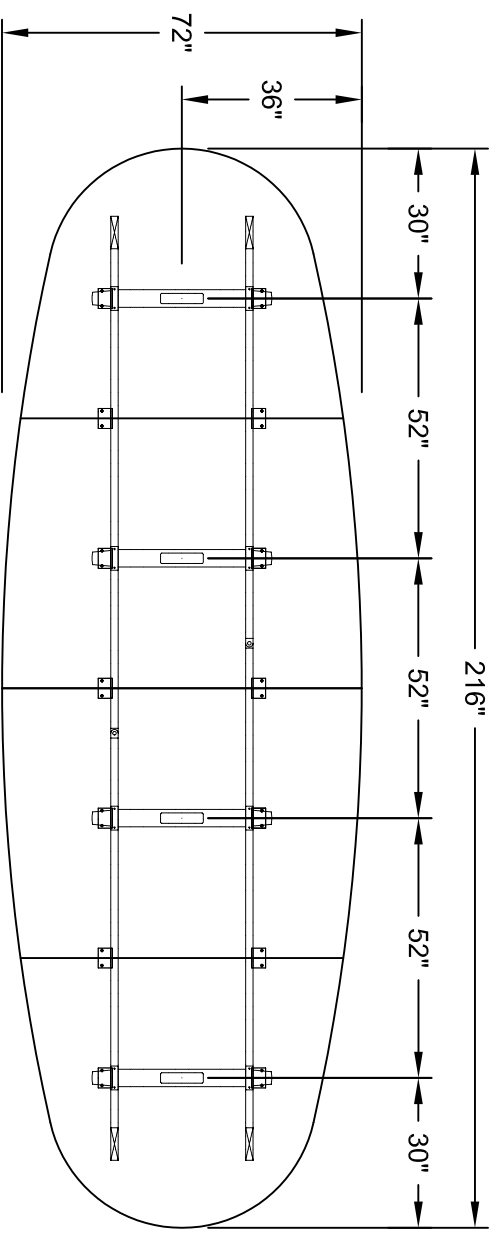
PLAN VIEW
