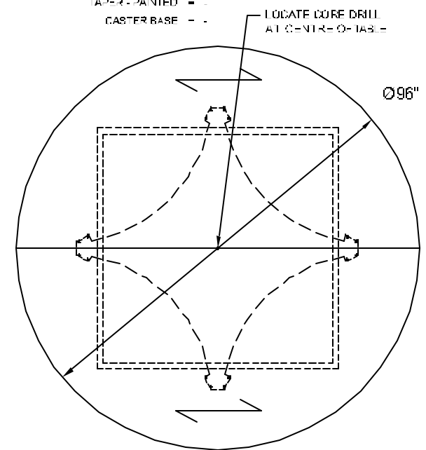
PLAN VIEW-QUAD BASE
