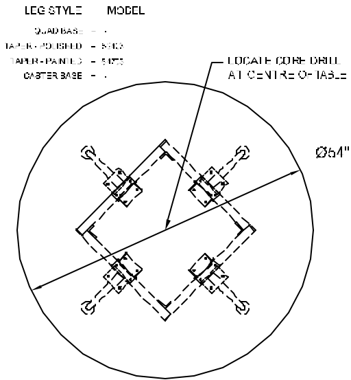
PLAN VIEW-TAPER BASE
