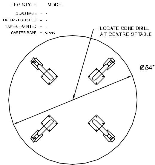
PLAN VIEW-CASTER BASE
