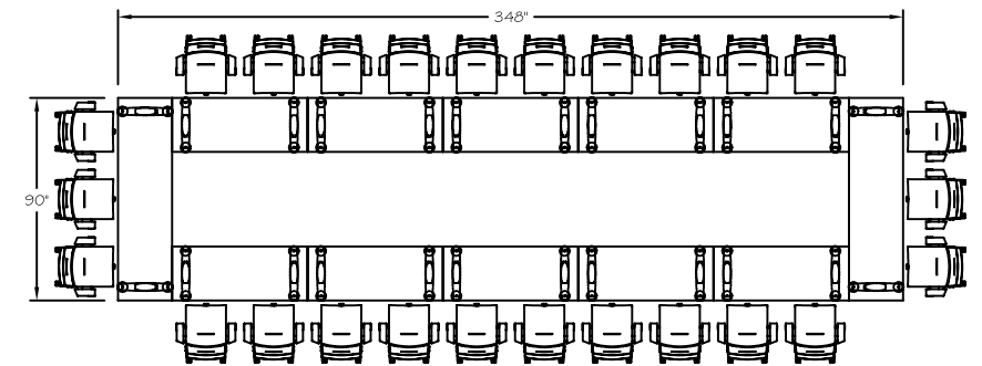
LAYOUT: FL-26-A1 6 @ 90° x 24" 4 @ 60° x 24"
