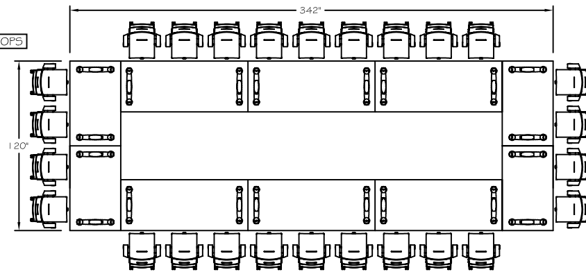
LAYOUT: FL-26-C1 6 @ 90° x 36" 4 @ 60° x 36"
