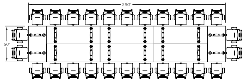
LAYOUT: IN-26-B1 6 @ 90° x 30" 2 @ 60° x 30"
