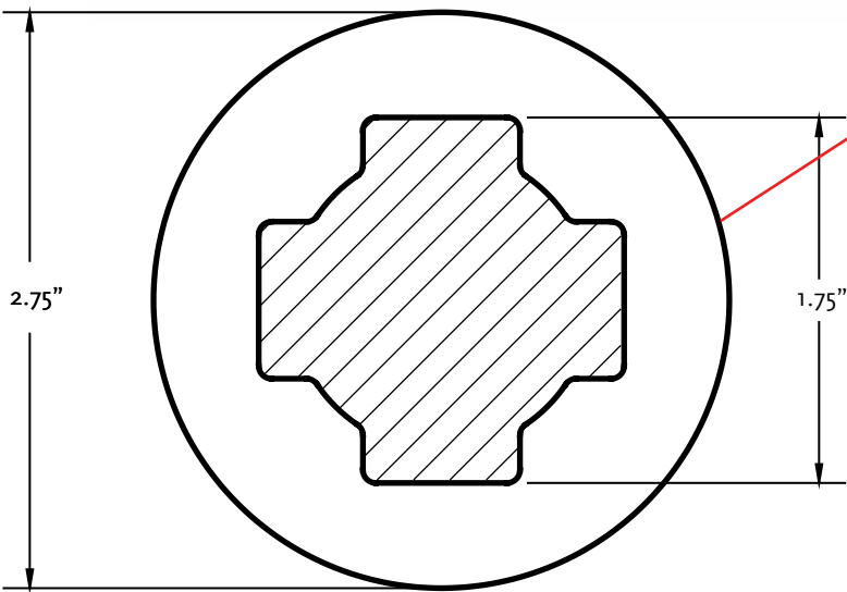
Cable access in base (full scale)
