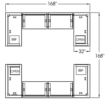
PLAN VIEW
