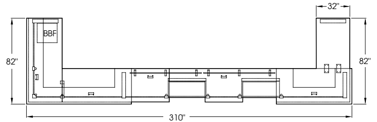
PLAN VIEW
