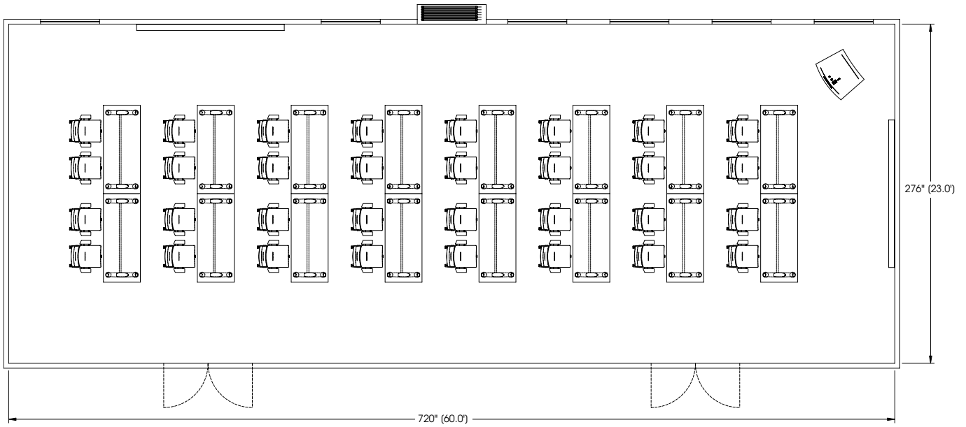
ROOM1-LAYOUT A3
