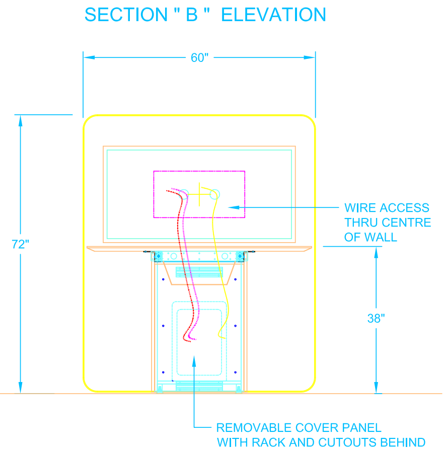
SECTION " B " ELEVATION
