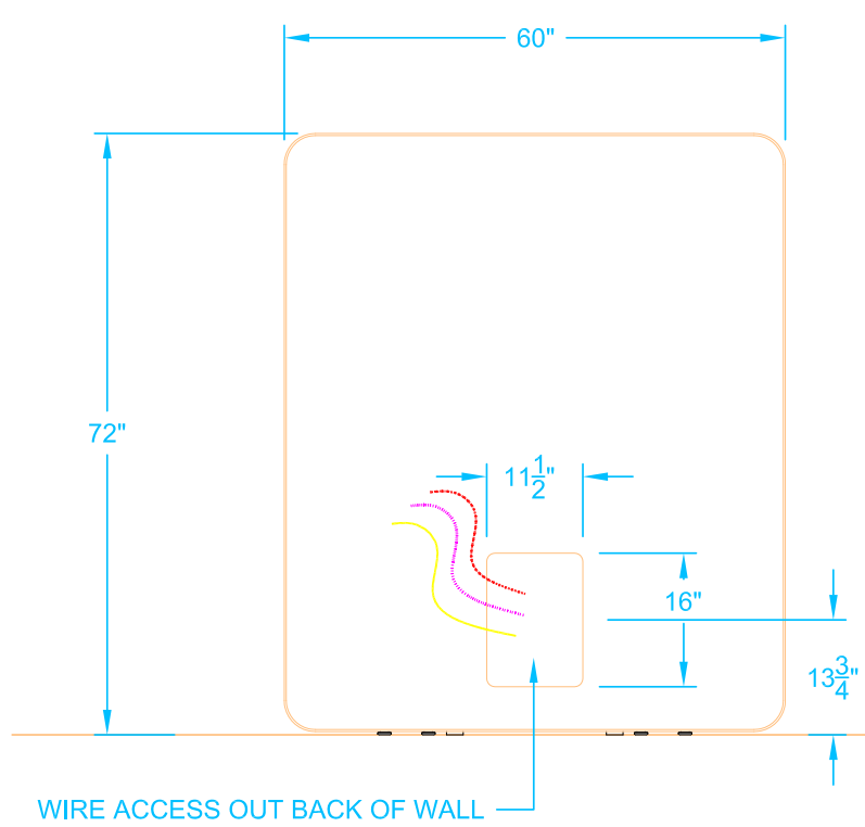
REAR ELEVATION
